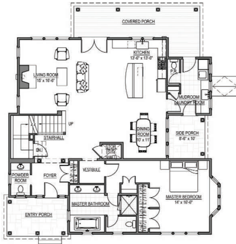
HOUSE F FIRST FLOOR PLAN - 1,857 G.S.F. SCALE: 1/8" = 1'-0"
