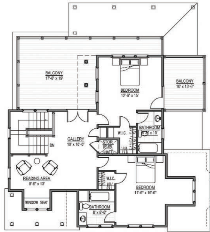
HOUSE F SECOND FLOOR PLAN - 1,084 G.S.F. SCALE: 1/8" = 1'-0"
